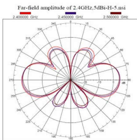
V-Plane Co-polarization
