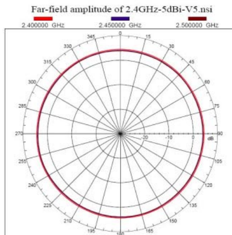
H-Plane Co-polarization
