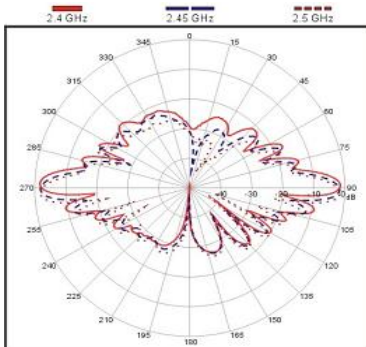
E-Plane Co-polarization 3-dB Beam width = 15°
