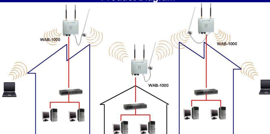
WAB-1000 Network Diagram
