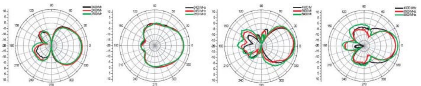
V-Plane Co-polarization
