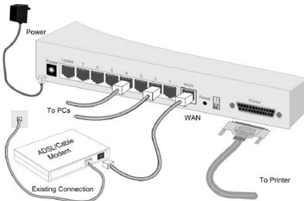
Figure 9: Installation Diagram
