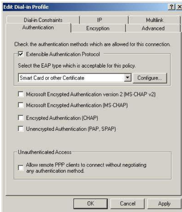
Figure 38: Authentication Screen
