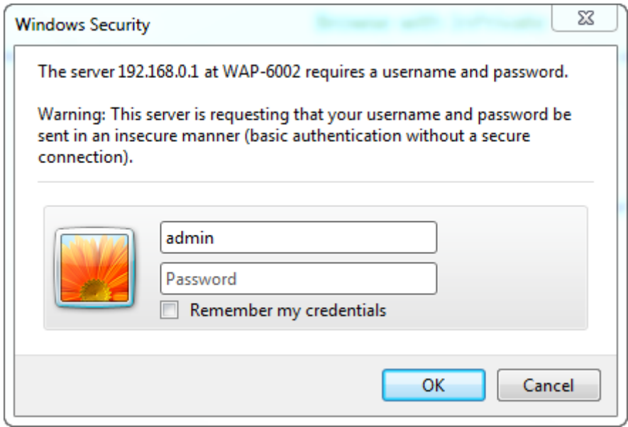
Figure 6: Password Dialog
