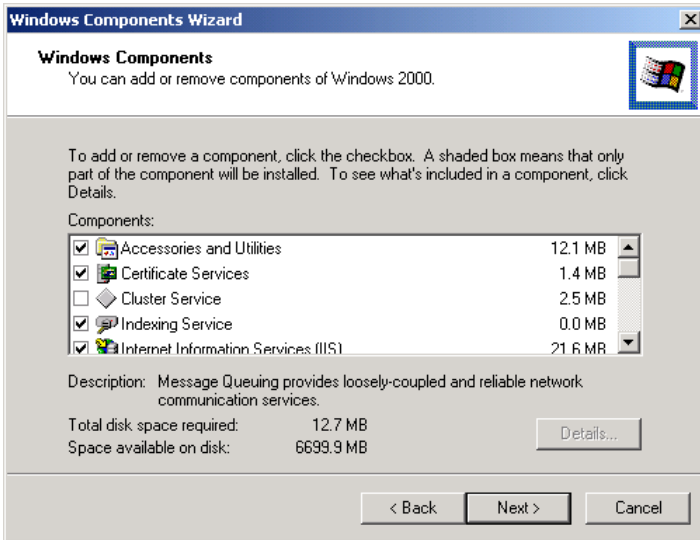
Figure 24: Components Screen
