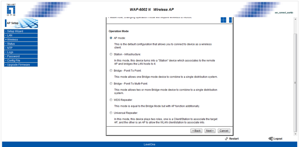
Figure 7: Home Screen
