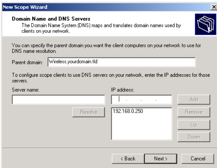
Figure 29: DNS Screen
