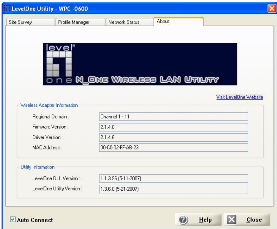
Figure 10: About Screen
