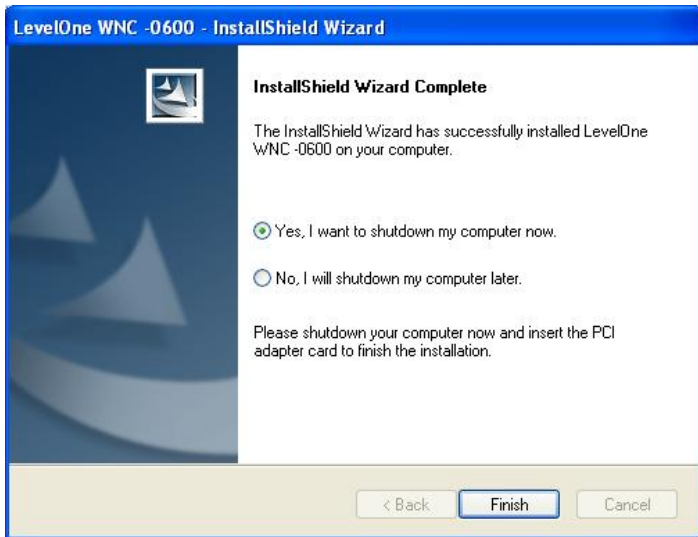
Figure 2: Installation Screen
