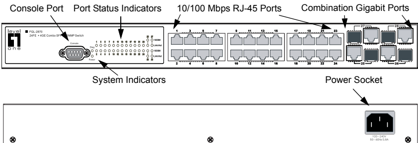
Figure 1-1. FGL-2870 Front and Rear Panels
